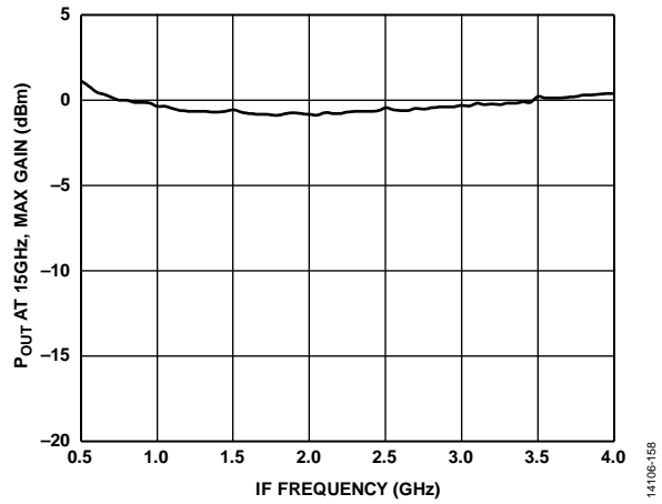
Figure 58. Bandwidth, P_{OUT} at 15 GHz and Maximum Gain Setting vs. IF Frequency ( f_{IF} )
