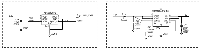
Figure 84. ADRF6780 Evaluation Board Schematic Page 2
