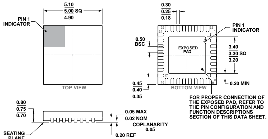
Figure 86. 32-Lead Lead Frame Chip Scale Package [LFCSP] 5 mm × 5 mm Body and 0.75 mm Package Height (CP-32-20) Dimensions shown in millimeters
