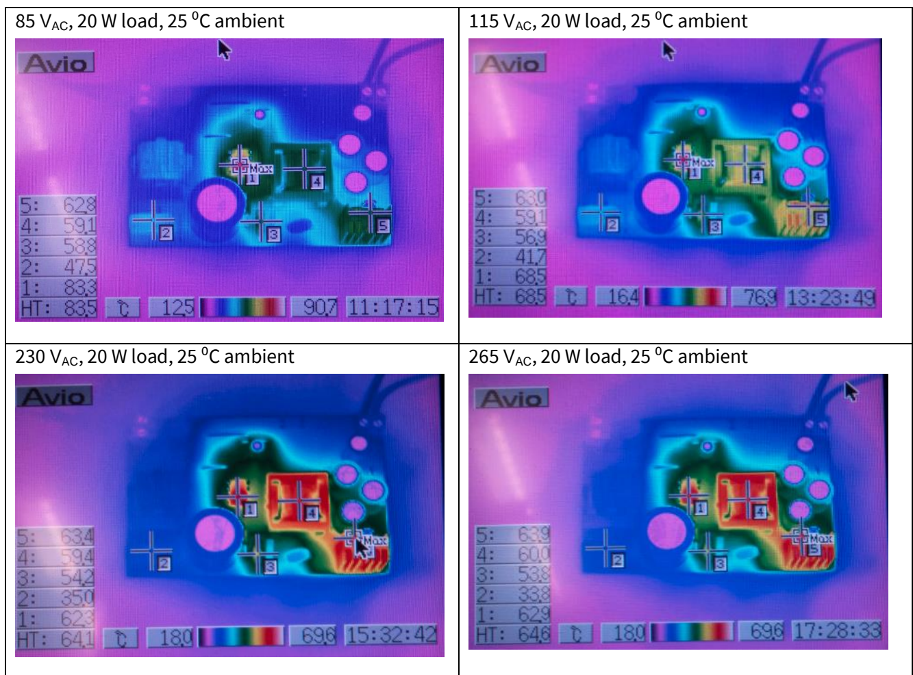
Figure 16 Infrared thermal image of EVAL ICE3AR2280VJZ
