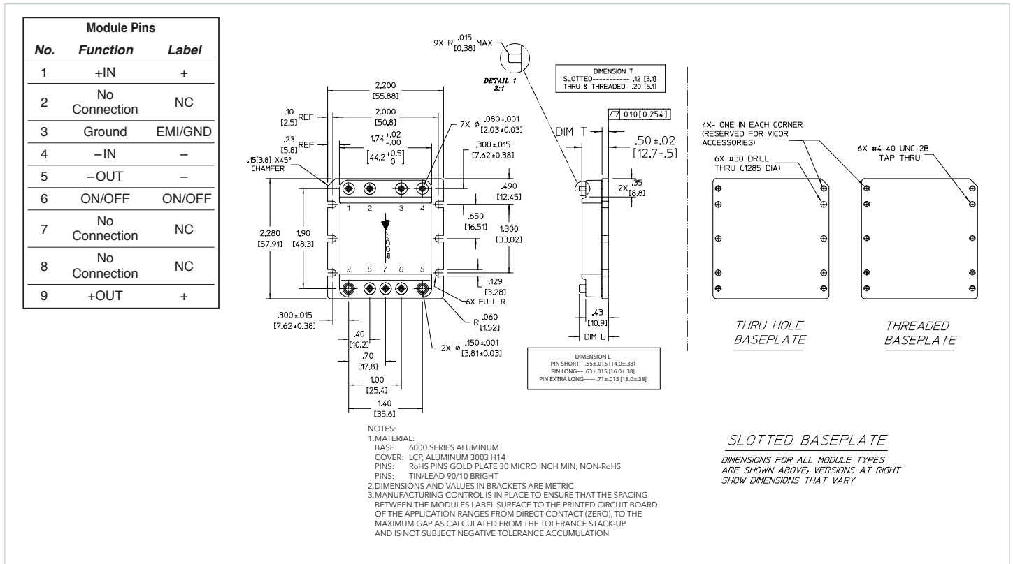
Figure 6 — Mechanical diagram
