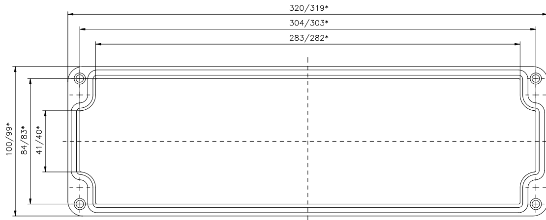
Deckel
