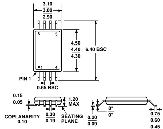
Figure 20. 8-Lead Thin Shrink Small Outline Package [TSSOP] (RU-8)
