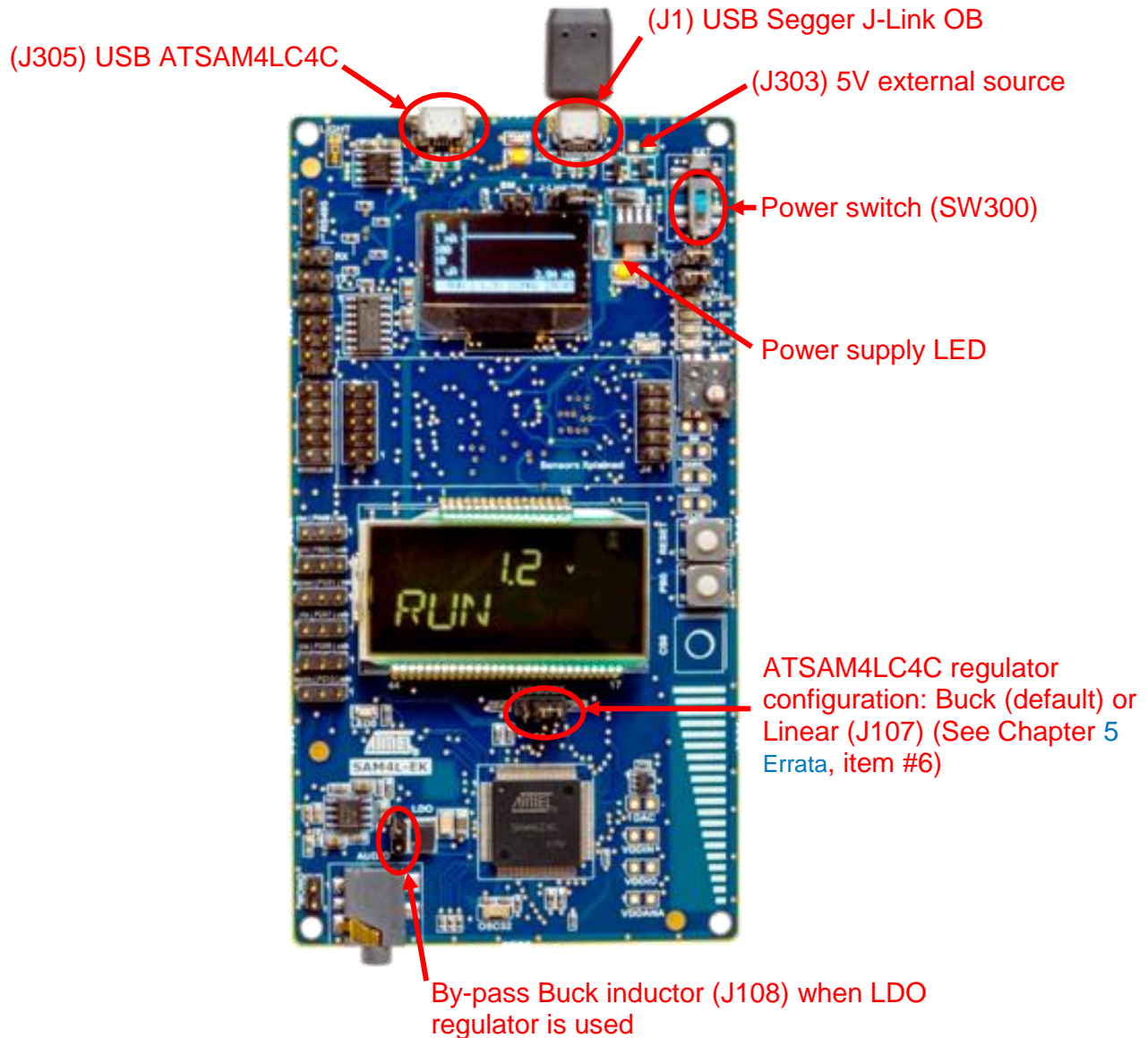
Figure 2-2. Power Supply Sources
