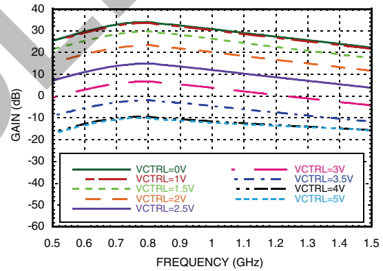
Gain vs. Frequency [2]
