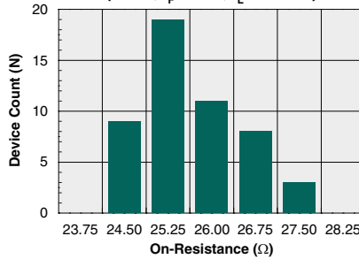
Typical On-Resistance Distribution (N=50, I F =0mA, I L =130mA)
