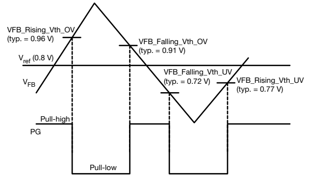
Fig. 9 - PGOOD Window
