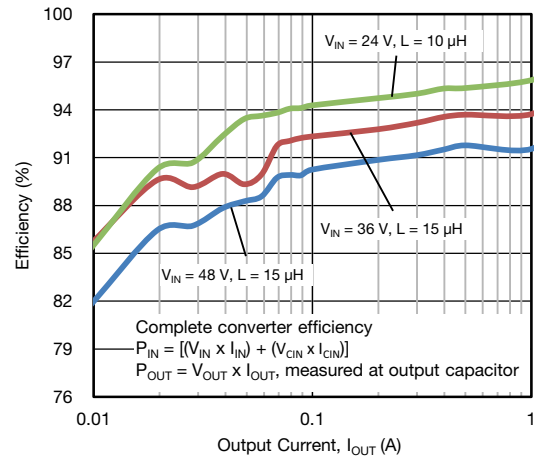
Fig. 21 - SiC462 Efficiency vs. Output Current - Light Load, V_{OUT} = 12\text{ V}
