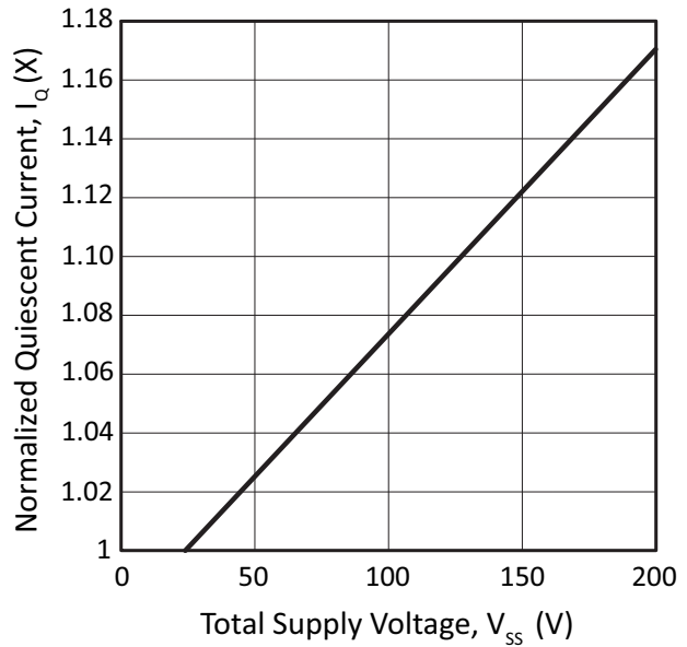
Figure 11: Quiescent Current
