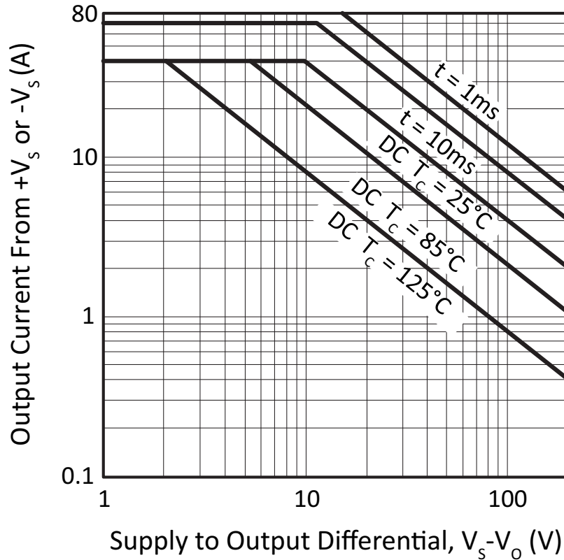
Figure 12: SOA
