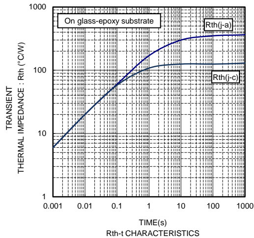
Rth-t CHARACTERISTICS
