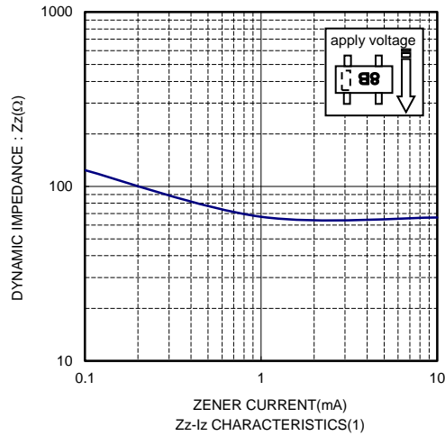
Zz-iz CHARACTERISTICS(1)
