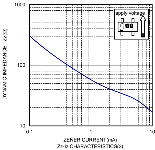
Zz-iz CHARACTERISTICS(2)
