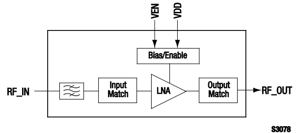
Figure 1. SKY65708-11 Block Diagram
