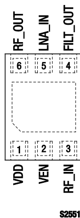
Figure 2. SKY65708-11 Pinout – 6-Pin MCM (Top View)
