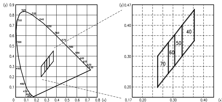
C.I.E. 1931 Chromaticity Diagram
