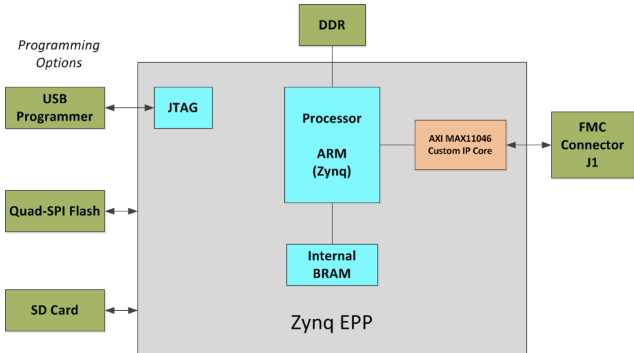
Figure 2. Block Diagram of FPGA Hardware Design
