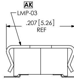
FIG 3 -P: PICK & PLACE PAD
